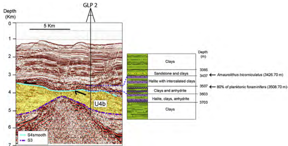
Figure 11. Zoom of Figure 8 showing onlap configuration of the strata that overlies S4smooth. These strata correspond with the evaporitic unit drilled by well GLP 2 (3703–3437 m depth). The (52 m thick) overlying sandstones and clays (3437–3385 m depth) are indistinct on the seismic profile. Depths are measured depths in meters below Kelly Bushing (mMDKB).
