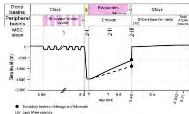
Figure 16. Variation of the Mediterranean Sea level in the Gulf of Lions between 6 and 5.30 Ma encompassing the MSC (augmented from Bache et al. (2012)). Successive major changes are estimated with respect to present-day sea level (0 m). The initial position of the paleoshoreline just before the rapid reflooding (step 2-III) has been estimated between 600 and 900 m below the present day sea level by Bache et al. (2012). The rapid increase in water depth during step 2-III was thus between 600 and 900 m. Solid and dashed black lines are constrained by an increase of 600 m and 900 m respectively. Subdivisions of the MSC shown on Figure 14.
