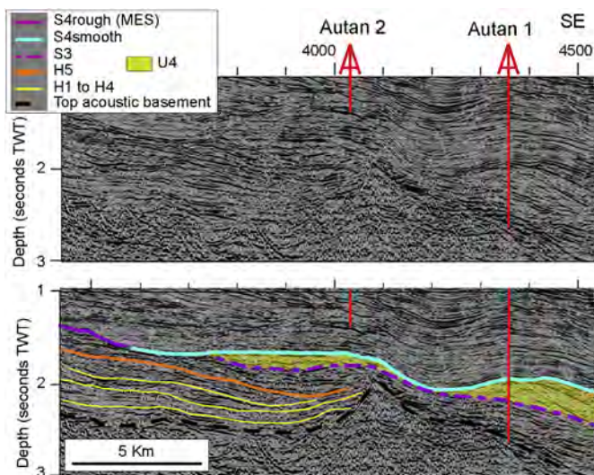
Figure 6. Zoom of Figure 4 showing the stratal relationship between U3 and U4 and the unconformity S3 that separates these units. Seismic reflectors H1 to H5 are older than U4. A Serravallian/Tortonian age for H5 leads to a younger age for the deposition of U4.
