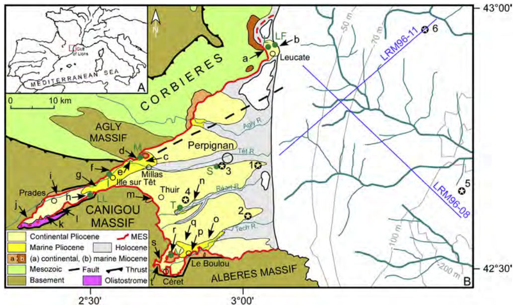
Figure 1. The Roussillon Basin. A, Map in the Western Mediterranean region. B, Simplified geological map of the Roussillon Basin showing the location of the offshore seismic profiles LRM96-08 and LRM96-11 and reconstructed Messinian fluvial network according to Lofi et al. (2003, 2005), Gorini et al. (2005) and Bache et al. (2009, 2012). Long wells used in this paper: 1, Canet 1; 2, Elne 1; 3, Mutualité agricole F1; 4, Ponteilla; 5, Rascasse 1; 6, Tramontane 1. Selection of sections studied: a, Codequas (Leucate); b, Trois Frères Cape (La Franqui); c, Saint-Martin (Millas); d, Poc Calbeil (Néfiach); e, Bente Farine (Néfiach); f, Les Orgues (Ille sur Têt); g, Les Escoumes (Vinça); h, La Lentilla (Marquixanes); i, Montcamill (Catlar); j, Coma del Mas (Serdinya); k, Saint-Eusèbe pass; l, Villerach; m, Rigall (Thuir); n, Ribèral (Trouillas); o, Les Forques (Banyuls dels Aspres); p, Moli Nou (Le Boulou); q, Pla del Rey (Tresserre); r, Els Pontells (Vivès); s, Mas Tauriac (Céret); t, Sant Pau chapel (Céret). Localities with mammal fauna: LL, La Lentilla; V, Vivès 2; M, Millas; I, Ille sur Têt; T, Terrats; S, Serrat d'en Vacquer; L, Leucate; LF, La Franqui. MES, Messinian Erosional Surface.
