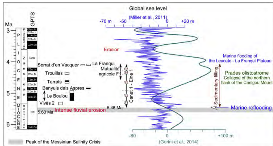
Figure 18. Chronostratigraphy of the events that affected the Roussillon Basin during the time interval 6–3 Ma, with respect to global changes in sea level. GPTS, Global Polarity Time Scale from Lourens et al. (2005).
