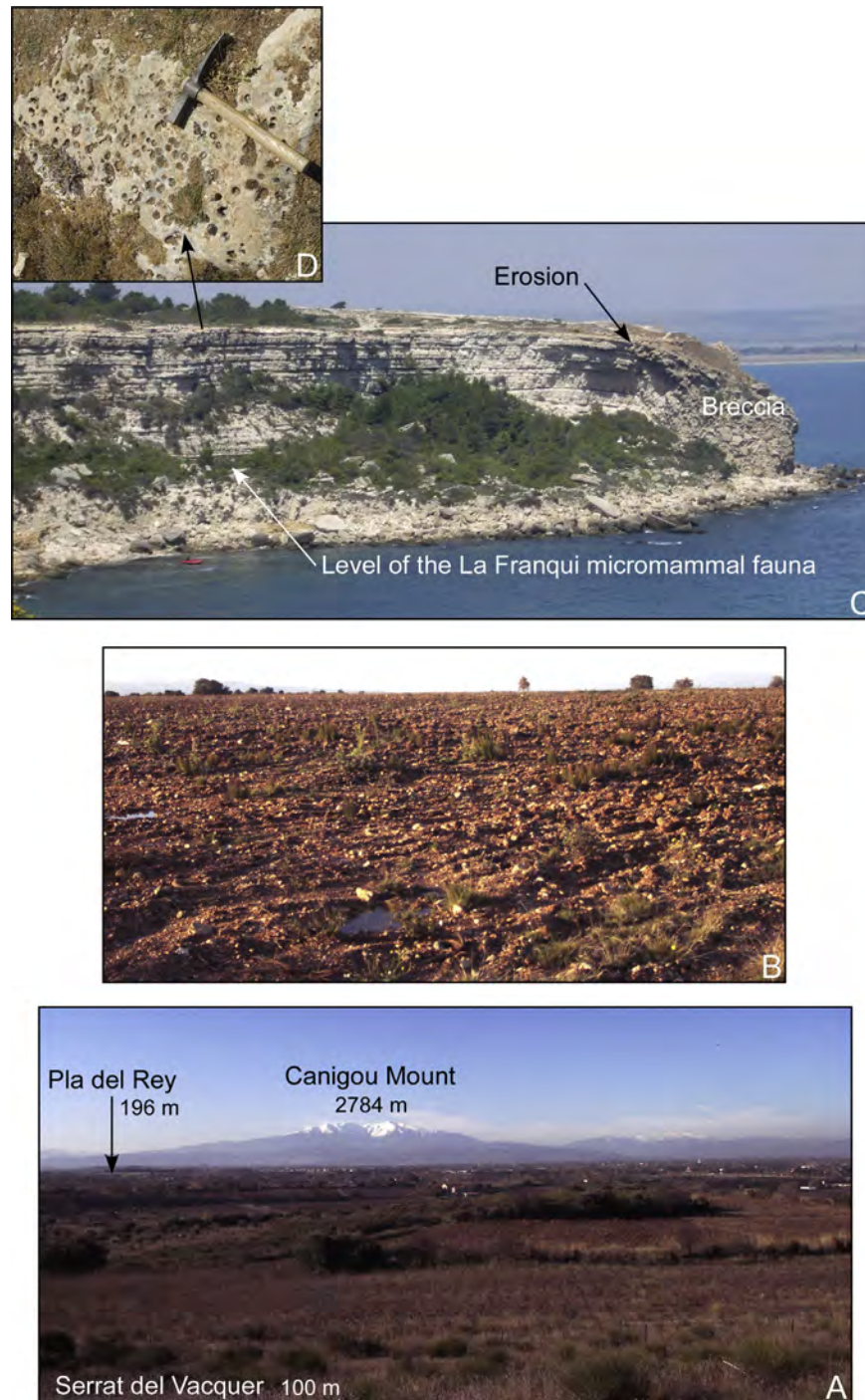
Figure 17. The surface topping the Roussillon Pliocene sedimentary filling. A, B, In its alluvial expression at Pla del Rey (Tresserre): A, View from the Serrat d'en Vacquer; B, Surface with siliceous pebbles and its red alteration (196 m asl). C, D, In its coastal expression at Trois Frères Cape (La Franqui): C, La Franqui section and the top surface (60 m asl) cut by Late Pliocene erosion; D, Burrows cut by saxicavous mollusks in the surface. (For interpretation of the references to colour in this figure legend, the reader is referred to the web version of this article.)
