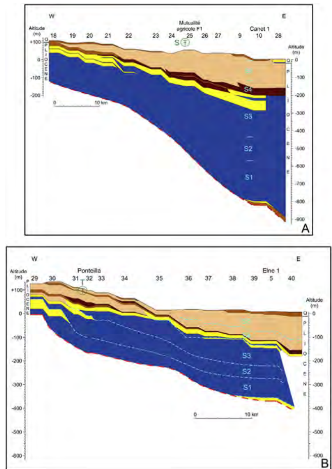
Figure 5. Geological transects of well sections across the Roussillon Basin (continued). Correlations of wells according to detailed logs and loggings (gamma ray and resistivity) are from Duvail (2008). Logs and loggings can be consulted on the website: http://infoterre.brgm.fr . Same legend and same explanations as for Figure 4. A, Longitudinal transect P2. S, Location of the Serrat d'en Vacquer mammal fauna. B, Longitudinal transect P3. T, Location of the Terrats (La Jasse) mammal fauna.
