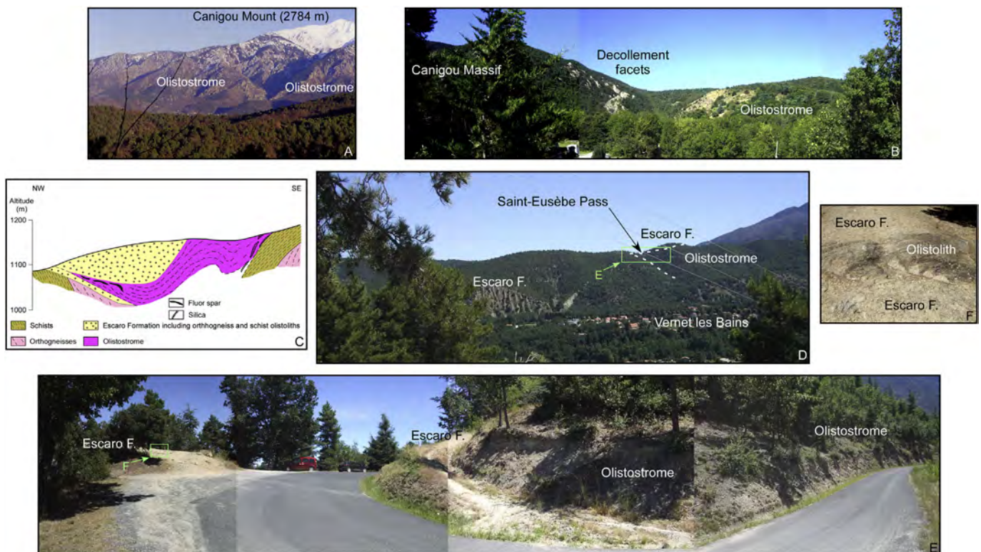
Figure 19. The Prades olistostrome. A, Overview of the olistostrome on the northern flank of the Canigou Massif. B, At Escaro, contact between the olistostrome and the Canigou orthogneisses marked by decollement facets. C, Section across the olistostrome, from Huard and Pelissonnier (1969). D, Overview of the Prades olistostrome sandwiched inside the Escaro Formation at the Saint-Eusèbe pass. E, Detail of the contact between the olistostrome and the Escaro Formation at the Saint-Eusèbe pass. F, At the Saint-Eusèbe pass, a block from the olistostrome incorporated within the sediments of the Escaro Formation.
