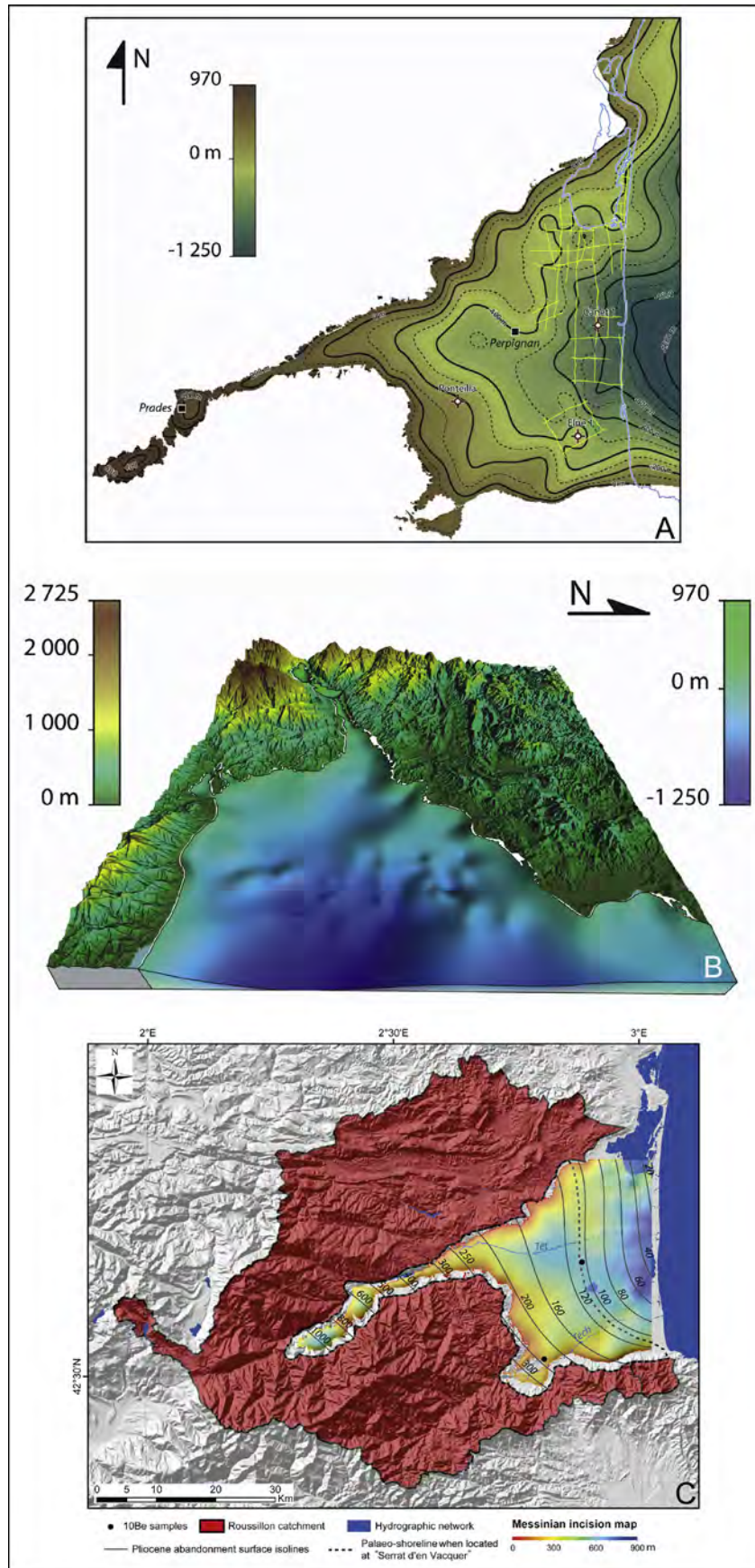
Figure 11. Reconstructed key surfaces in the Roussillon Basin. A, Current depth map (above and below sea level) of the MES in the Roussillon Basin. The seismic lines used for the modeling process are drawn in yellow. The map also shows the locations of the three main wells. B, Three-dimensional representation of the MES in the Roussillon Basin showing the two main eastward fluvial incisions. C, Map of the reconstructed Pliocene abandonment surface over the Messinian incision map in its hydrologic setting. The red area corresponds to the catchment feeding the Pliocene rias. The black dots show the location of the 10Be samples used to estimate the Pliocene denudation rate. The solid black lines are isolines corresponding to the reconstructed elevation of the Pliocene post-filling surface. The dashed line shows the expected location of the palaeo-shoreline when it was located at “Serrat d’en Vacquer”. (For interpretation of the references to color in this figure legend, the reader is referred to the web version of this article.)
