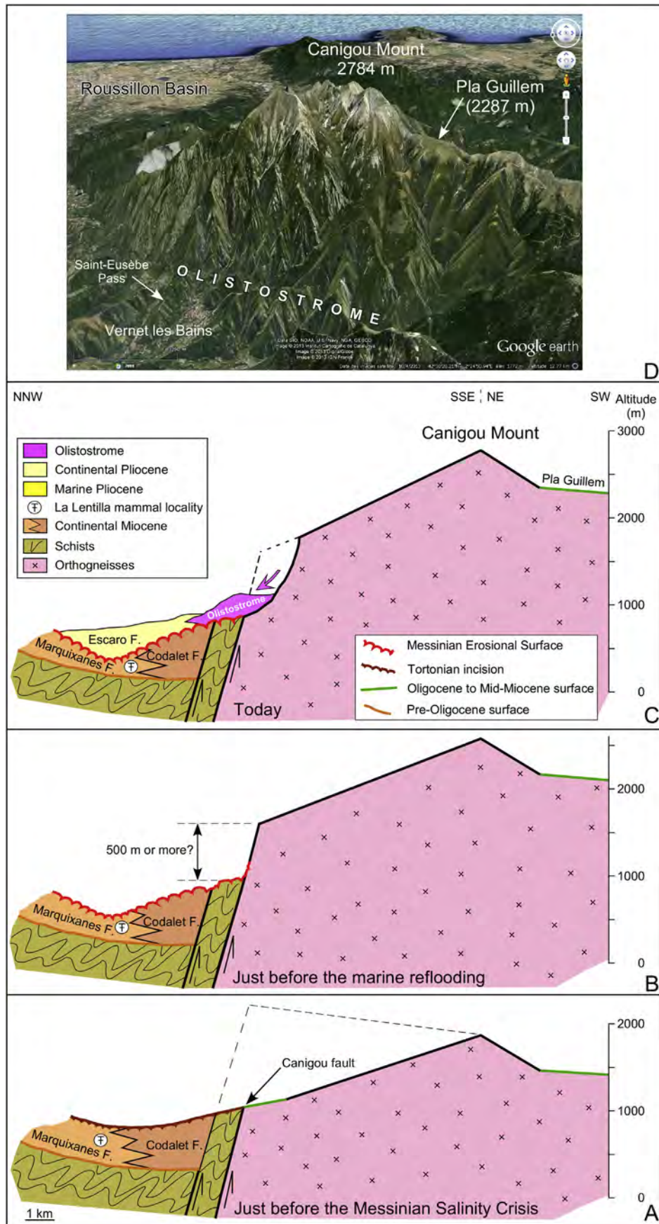
Figure 20. Evolution of the northern flank of the Canigou Massif since 6 Ma. A, Before the Messinian Salinity Crisis. The palaeoaltitude is estimated. B, After the peak of the Messinian Salinity Crisis, just before the marine reflooding of the Mediterranean basin but just after reactivation of the Canigou fault. C, Present-day relationships among the units and geometries, particularly with regard to the Prades olistostrome. D, Three-dimensional Google earth view of the Canigou Massif from its northern flank, with location of the Prades olistostrome and the uplifted Oligocene–Miocene surface (Pla Guillem). Elevation is three times exaggerated.
