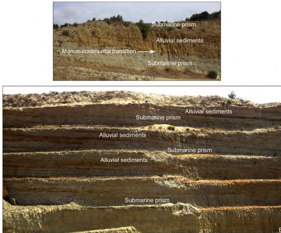
Figure 14. Sedimentary prisms at Bente Farine (Néfiach).
