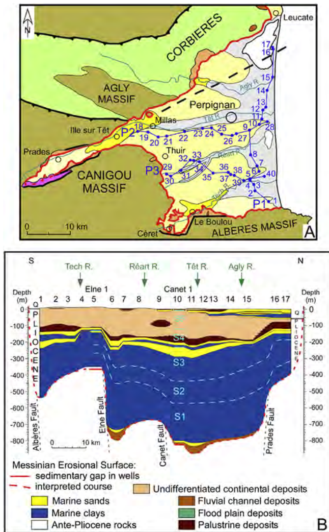
Figure 4. Geological transects of well sections across the Roussillon Basin. A, Map showing the location of the three transects (P1, P2, P3). Well numbers refer to Table 1. B, Transverse transect P1. Correlations of wells according to detailed logs and loggings (gamma ray and resistivity) are from Duvail (2008). Logs and loggings can be consulted on the website: http://infoterre.brgm.fr . S1 to S5, Sedimentary sequences (separated by dotted light blue lines); Q, Quaternary. (For interpretation of the references to color in this figure legend, the reader is referred to the web version of this article.)
