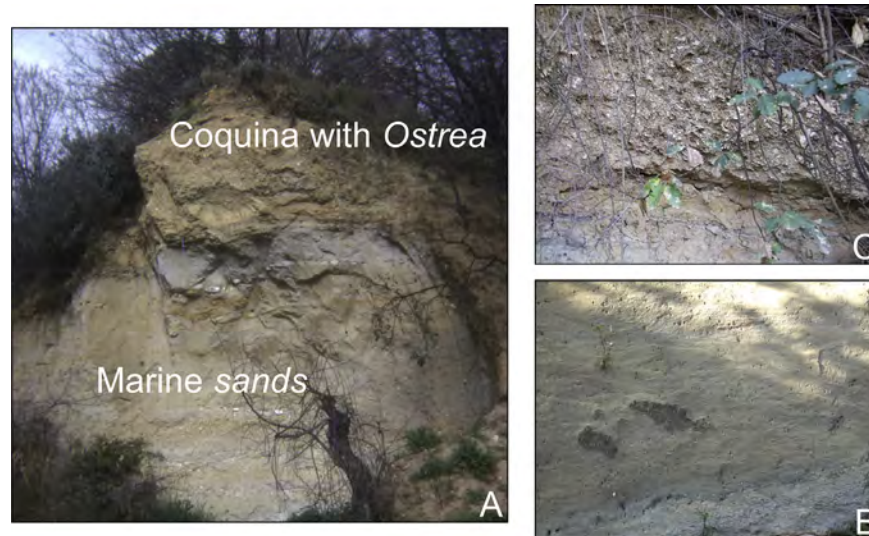
Figure 15. The Ribèral section at Trouillas. A, Complete view of the section. B, Marine sands with tide ripple marks. C, Coquina with Ostrea cucullata .
