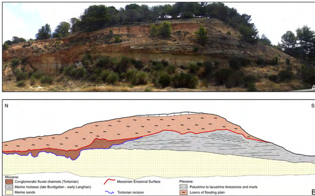
Figure 6. The Codequas section near Leucate. A, Panoramic photograph of the section. B, Its geological interpretation.
