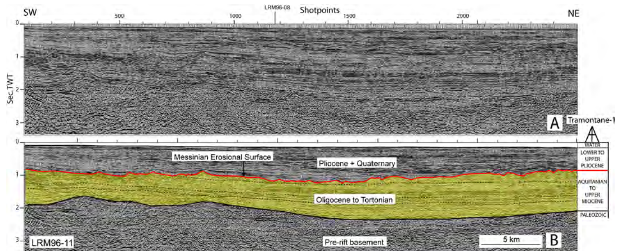
Figure 3. Interpreted and uninterpreted seismic profile LRM96-11 across the Gulf of Lions tied to Tramontane-1 well. The erosional surface observed offshore Roussillon truncates Upper Miocene sediments and is covered by sediments from the earliest stage of the Pliocene (Cravatte et al., 1974; Guennoc et al., 2000) supporting the hypothesis that this unconformity corresponds to the Messinian Erosional Surface. The location of the seismic profile is shown in Figure 1.
