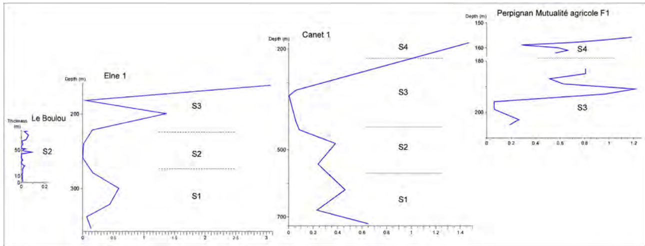
Figure 16. Comparison of the “Halophytes/ Pinus ” pollen ratio in the long sections Le Boulou, Elne 1, Canet 1 and Mutualité agricole F1. S1 to S4, Sedimentary sequences located in Figures 4B and 5.
