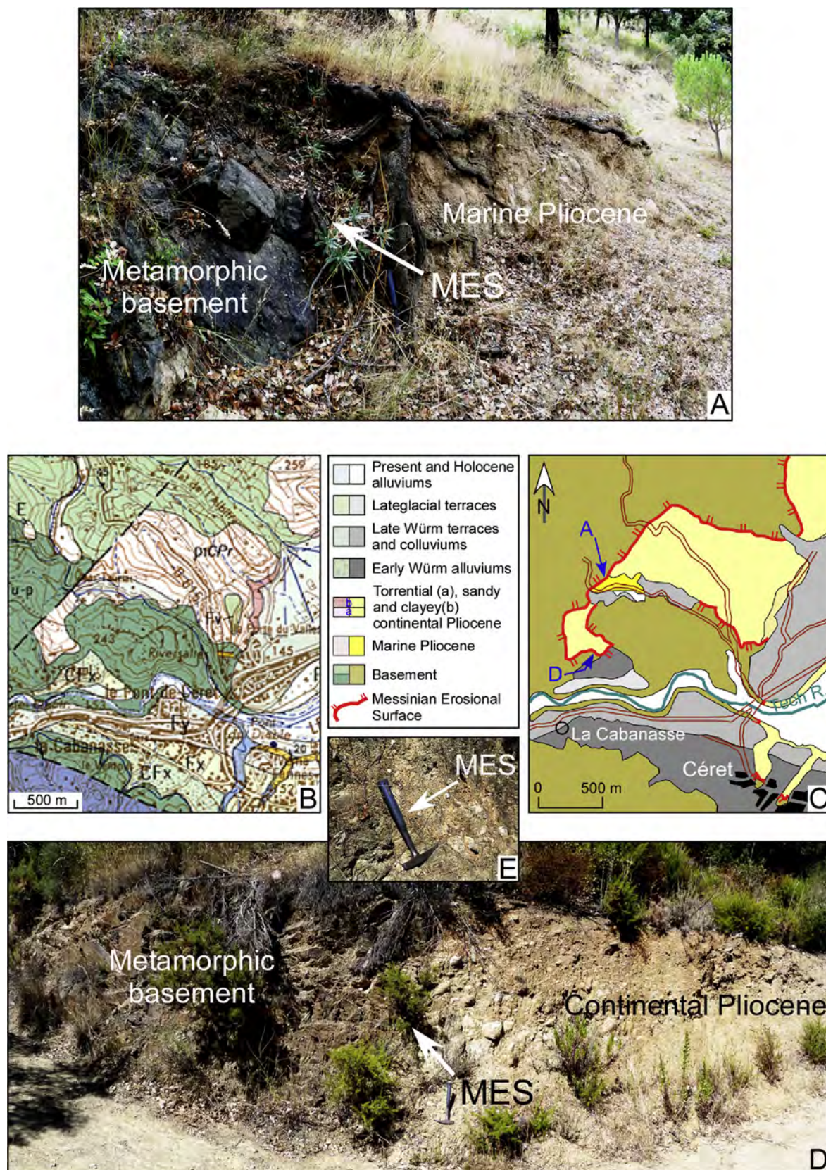
Figure 10. The Messinian Erosional Surface in the area of Céret. A, View of the Messinian Erosional Surface at Mas Tauriac. B, Part of the Céret geological map ( http://www.infoterre.fr ; map 1096). C, Detail of our geological map showing the location of the photograph shown in Figures A and D. D, View of the Messinian Erosional Surface at the Sant Pau chapel. E, Detail of the MES at the Sant Pau chapel. Of the two symbols in the legend: the left one concerns the Céret B.R.G.M. map (Fig. B), the right concerns the authors' map (Fig. C).
