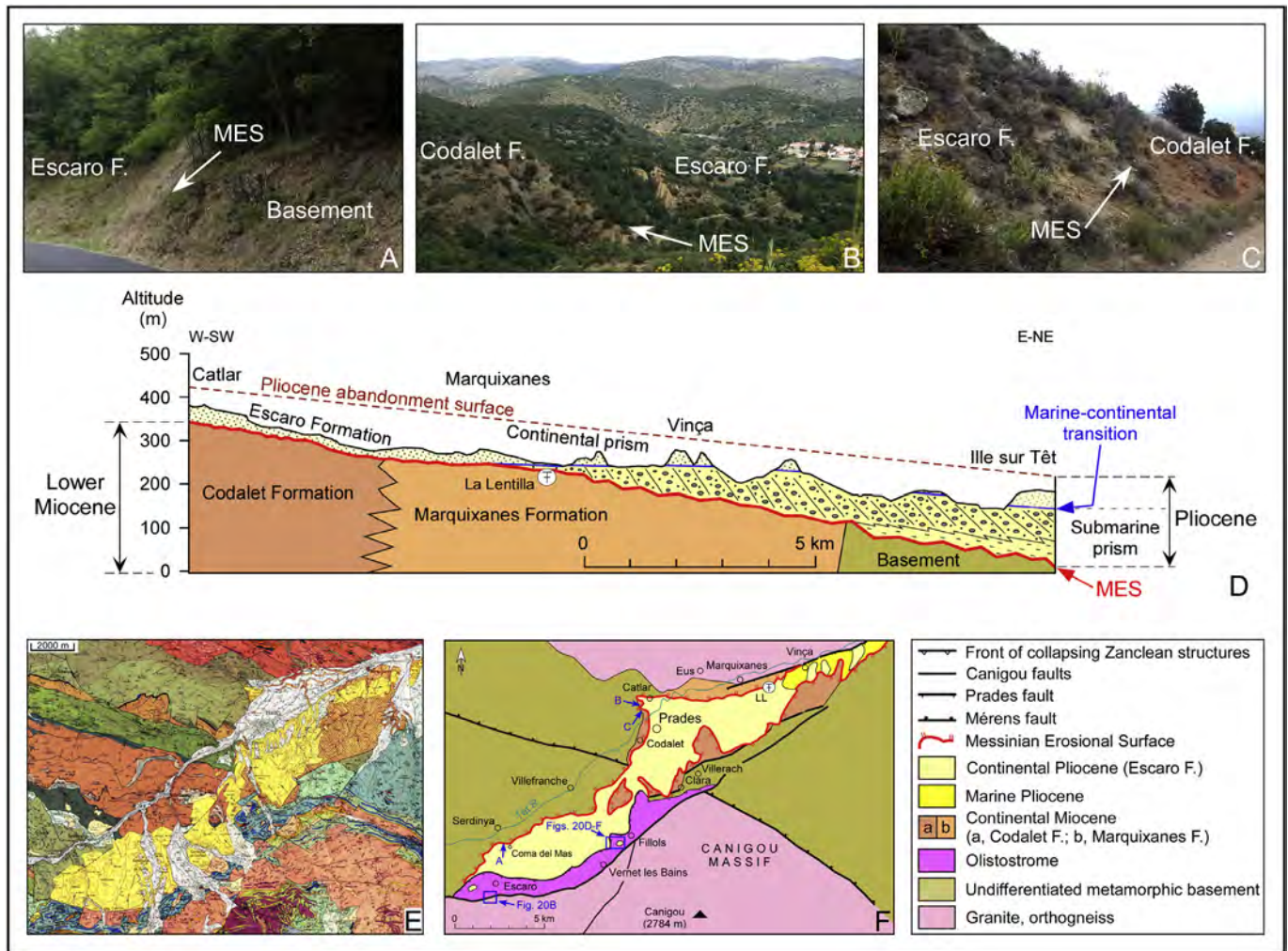
Figure 8. The Messinian Erosional Surface in the area of Prades (Conflent territory). A, View of the Messinian Erosional Surface at Coma del Mas (Serdinya), locality A in Figure F. B, View of the Messinian Erosional Surface at Montcamill (Catlar), locality B in Figure F. C, View of the Messinian Erosional Surface at Montcamill (Catlar), locality C in Figure F. D, W–SW – E–NE cross-section from Catlar to Ille sur Têt. E, Part of the geological map of Prades (Guitard et al., 1998). The color codes are explained in the legend of the map. F, The authors' geological map of the Conflent. A, Coma del Mas (Serdinya); B and C, Montcamill (Catlar); LL, Location of mammal fauna at La Lentilla; the blue rectangle shows the location of Figure 19. (For interpretation of the references to color in this figure legend, the reader is referred to the web version of this article.)
