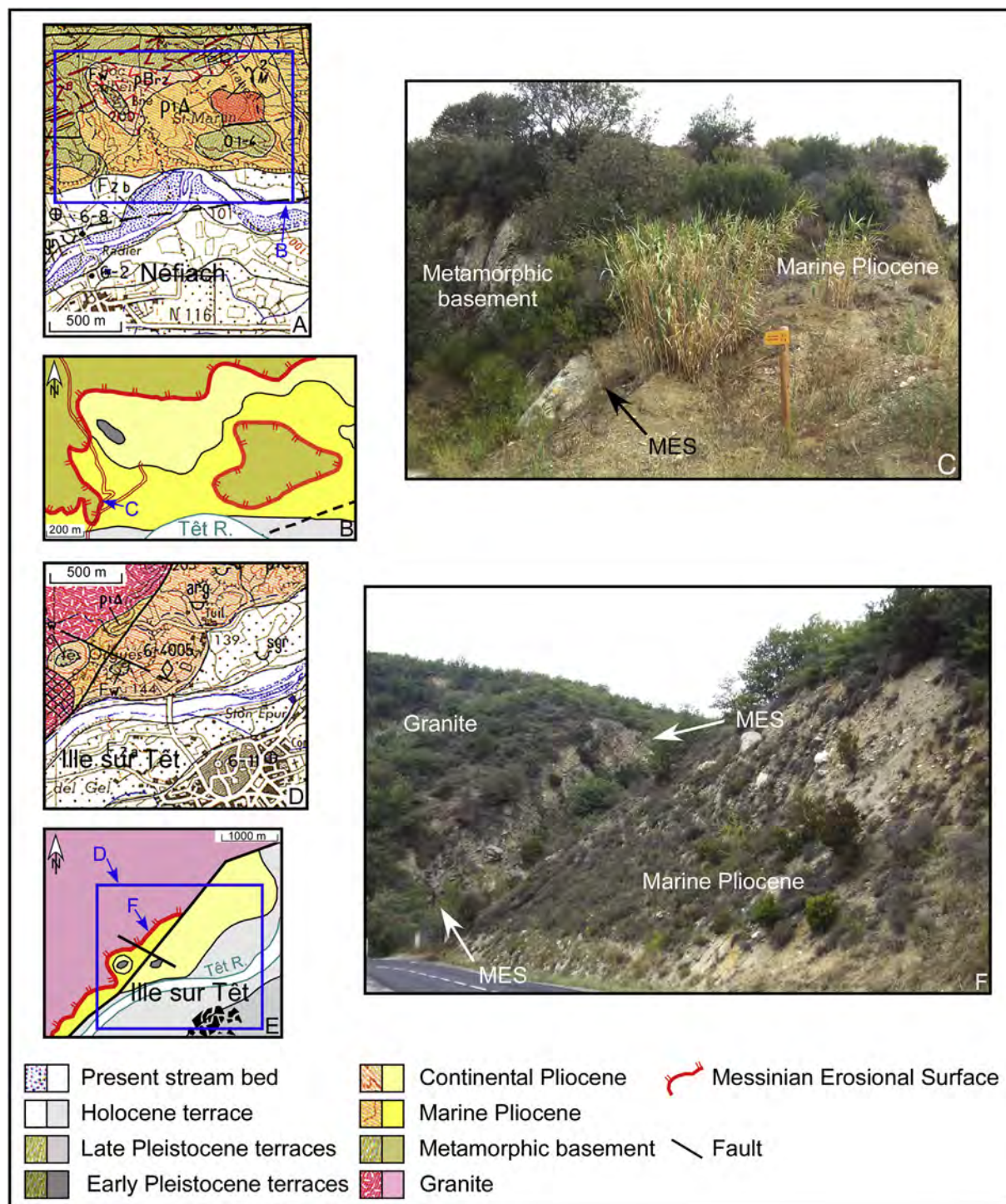
Figure 7. The Messinian Erosional Surface in the area of Nèfiach – Ille sur Têt. A, Part of the geological map of Rivesaltes (Berger et al., 1993) showing the location of the map detailed in Figure B. B, Detail of the geological map published by Clauzon (1990) and Clauzon et al. (1990) showing the location of the photograph in Figure C. C, View of the Messinian Erosional Surface at Poc Calbeil (Nèfiach). D, Part of the geological map of Rivesaltes (Berger et al., 1993). E, Detail of the geological map published by Clauzon (1990) and Clauzon et al. (1990) showing the area covered by Figure D and the location of the photograph in Figure F. F, View of the Messinian Erosional Surface at Les Orgues (Ille sur Têt). Of the two symbols in the legend: the left one concerns the Rivesaltes B.R.G.M. map (Figs. A and D), the right one concerns the Clauzon's maps (Figs. B and E).
