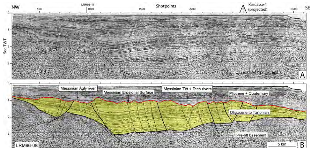
Figure 2. Interpreted and uninterpreted seismic profile LRM96-08 across the Gulf of Lions showing the unconformity that erodes faulted and relatively parallel strata. Mapping of this unconformity revealed a pattern of up to 5th order dendritic drainage with two main systems (Fig. 1) (Genesseeux and Lefebvre, 1980; Guennoc et al., 2000; Lofi et al., 2005; Bache et al., 2009). The two systems were mapped upstream in the Languedoc-Roussillon region and in the Rhône Valley where erosion is observed up to at least 350 km from the present coast (Clauzon, 1978, 1979, 1982). This unconformity is commonly interpreted as a subaerial erosional surface (the Messinian Erosional Surface) sculpted during the main MSC fall in sea level (Ryan and Cita, 1978; Guennoc et al., 2000; Lofi et al., 2005; Bache et al., 2009). The location of the seismic profile is shown in Figure 1.
