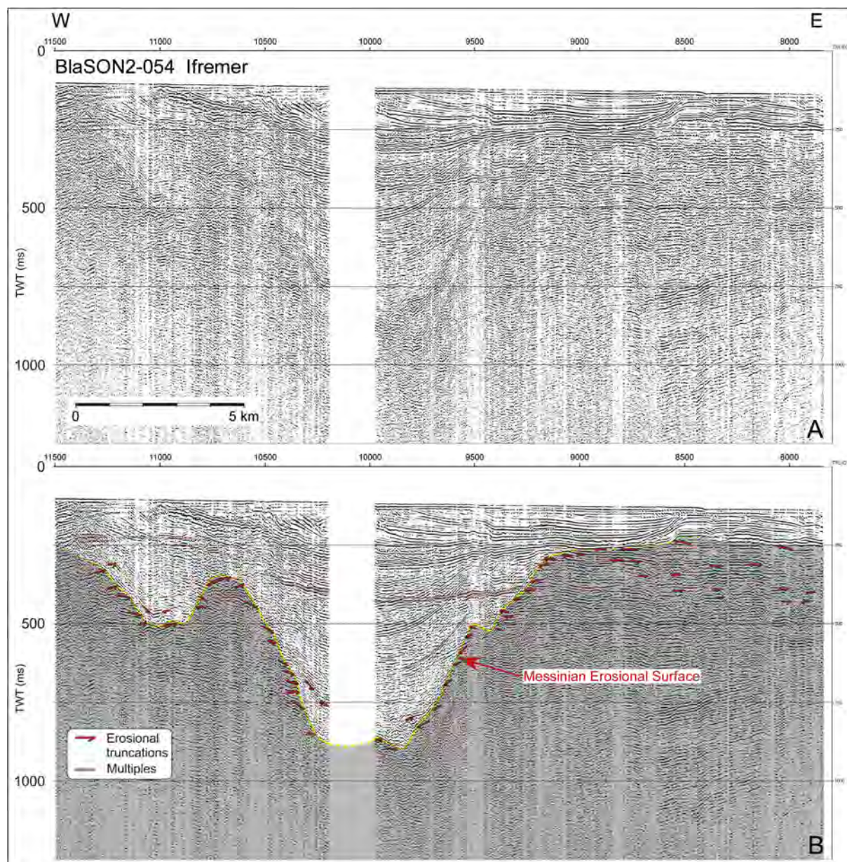
Figure 9. Seismic profile BlaSON2-054. A, Non interpreted profile. B, Interpreted profile.
