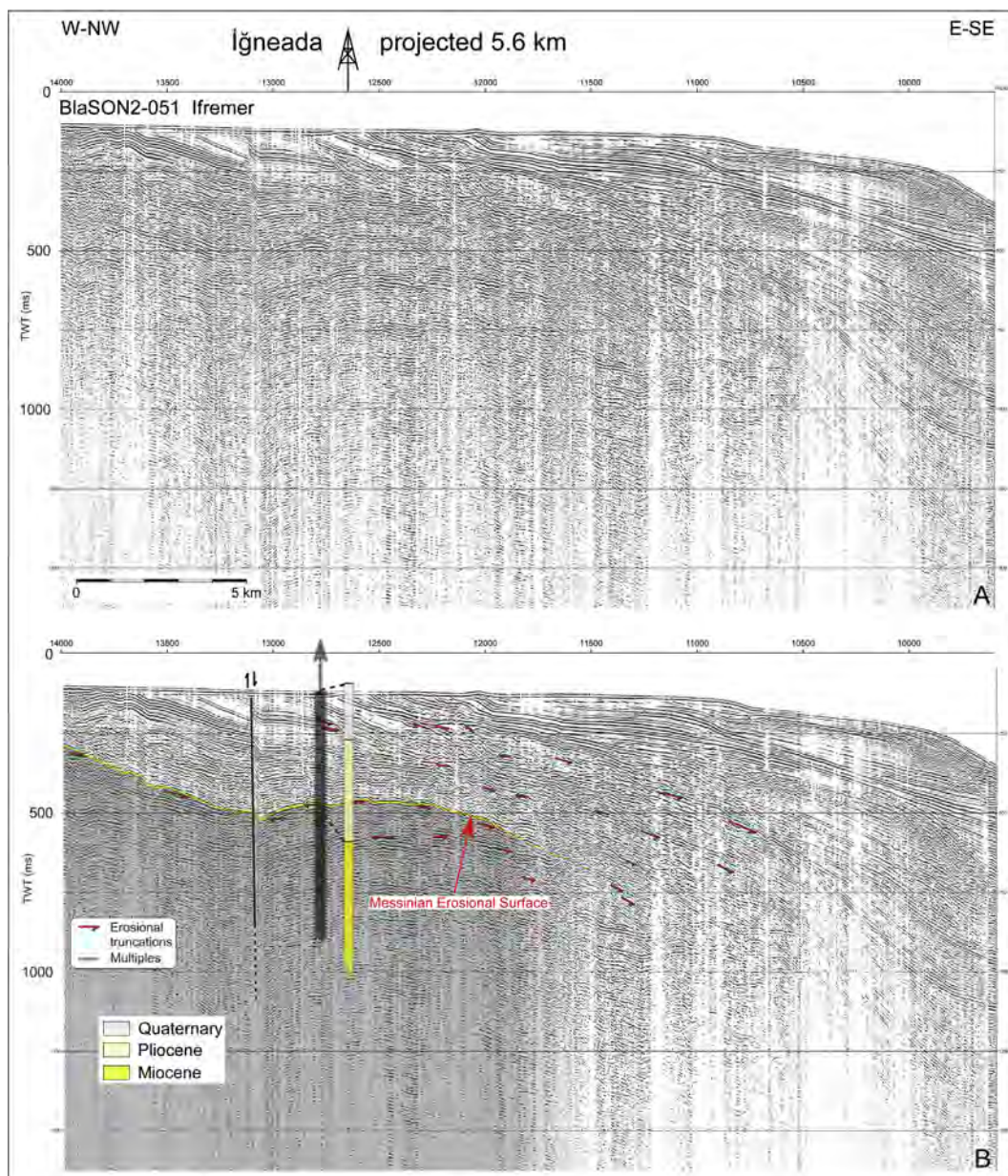
Figure 11. Seismic profile BlaSON2-051. A, Non interpreted profile with location of the projected İğneada 1 well. B, Interpreted profile with stratigraphic subdivision of the projected İğneada 1 well.
