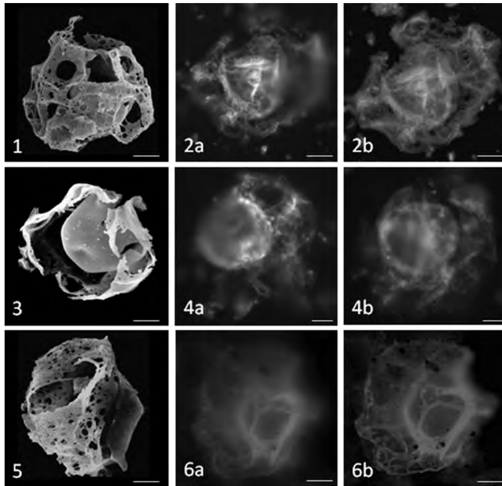
Plate 1. Dinoflagellate cysts of the Galeacysta etrusca Complex recorded in the Aragonite and Black shales units of Site 380 compared to reference specimens. Bar scale: 20 \mu\text{m} . Figure 1. Galeacysta etrusca , reference specimen from Krajačići at the scanning electronic microscope (latest Tortonian, Pannonian Basin; Popescu et al., 2009). Figures 2a, 2b. Galeacysta etrusca , Site 380 (1009.36 m) in fluorescence microscopy. Figure 3. R. areolatum , reference specimen from Majs 2 at the scanning electronic microscope (late Tortonian, Pannonian Basin; Popescu et al., 2009). Figures 4a, 4b. R. areolatum , Site 380 (1009.36 m) in fluorescence microscopy. Figure 5. S. balcanicus , reference specimen from Hinova at the scanning electronic microscope (latest Messinian, Dacic Basin; Popescu et al., 2009). Figures 6a, 6b. S. balcanicus , Site 380 (846.14 m) in fluorescence microscopy.
