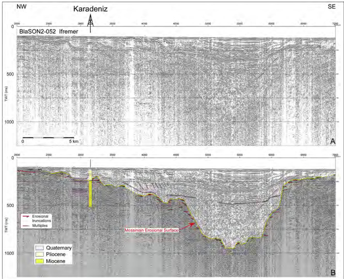
Figure 10. Seismic profile BlaSON2-052. A, Non interpreted profile with location of the Karadeniz 1 well. B, Interpreted profile with stratigraphic subdivision of the Karadeniz 1 well.
