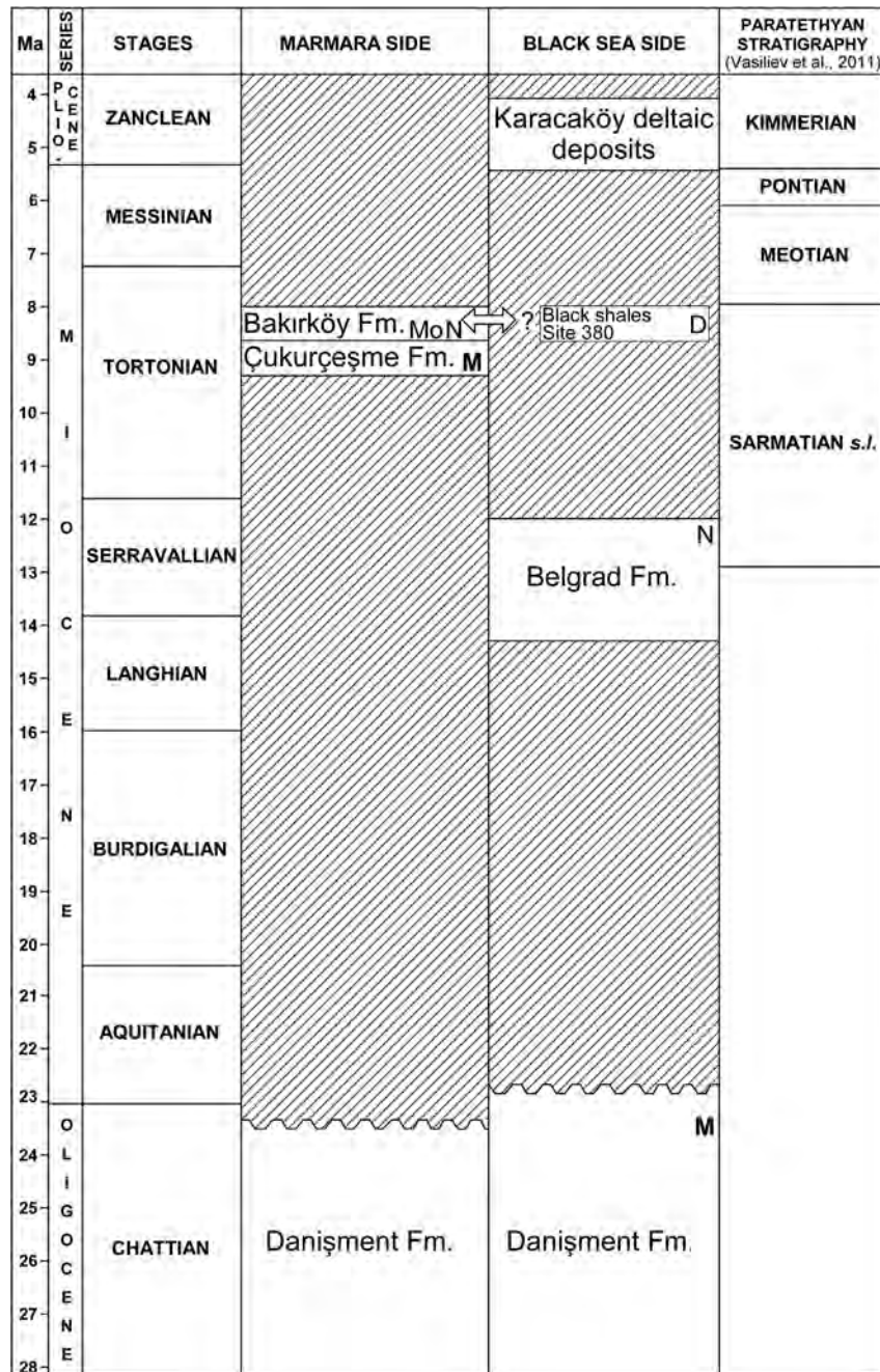
Figure 12. Interpreted onland stratigraphic successions on both sides of the Strandja Sill. Reference to the Paratethys Stratigraphy is done for the time interval corresponding to its more or less continuous isolation, i.e. from the early Sarmatian s.l. (= mid-Serravallian) to Kimmerian (= Zanclean). M, Mammals; N, Calcareous nannofossils; Mo, Molluscs; D, Dinoflagellate cysts. Double arrow: possible marine connection. Hatched areas: sedimentary gaps.
