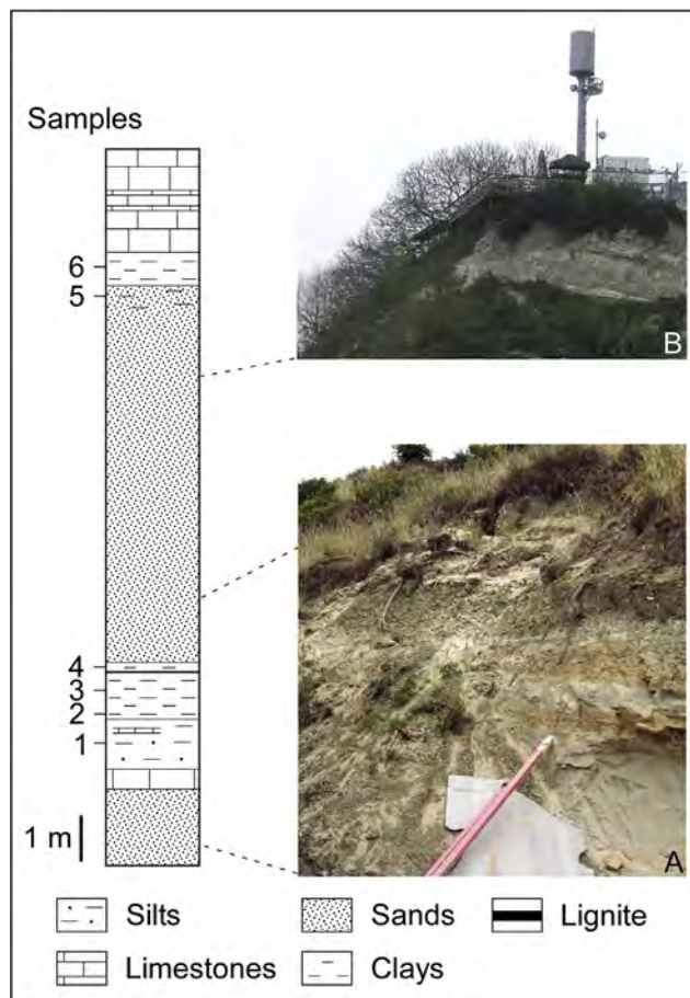
Figure 4. The Avclar section. 1 to 6, samples. A, Lower part of the section. B, Upper part of the section.
