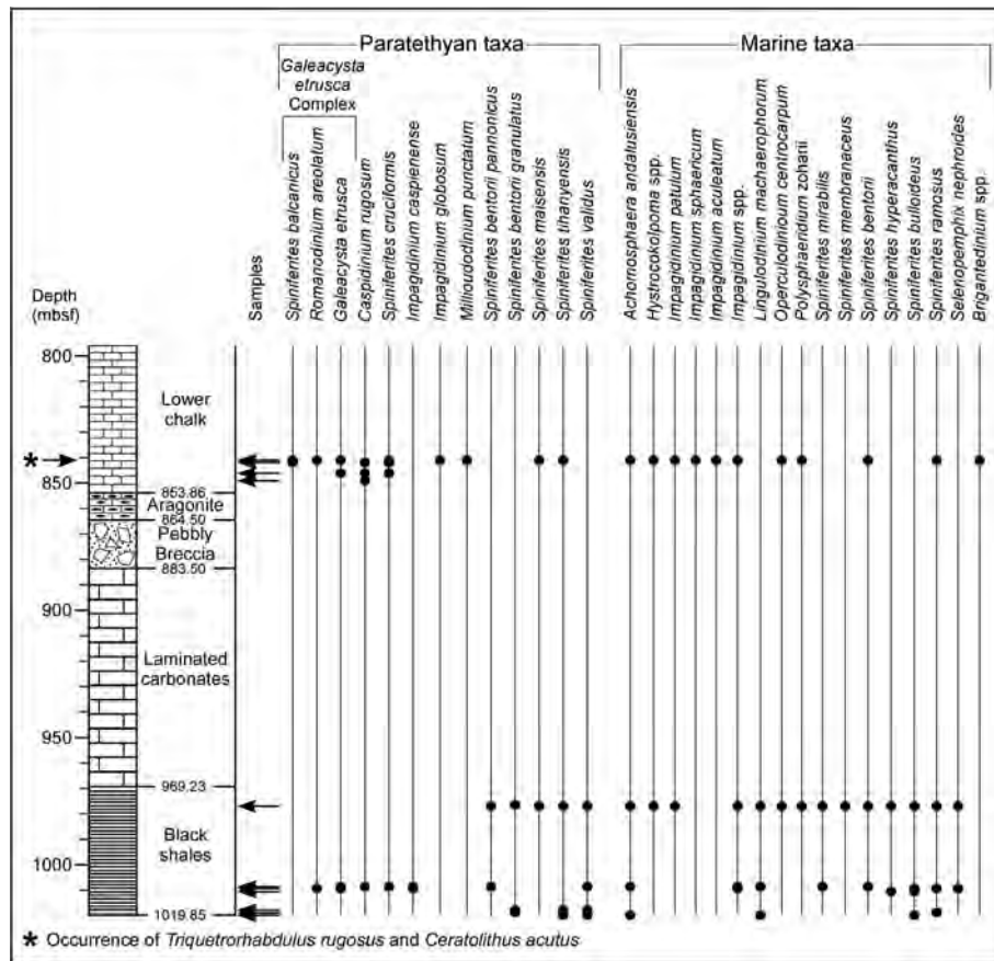
Figure 8. Dinoflagellate cyst content from the interval 840.07–1019.85 m of DSDP Site 380.
