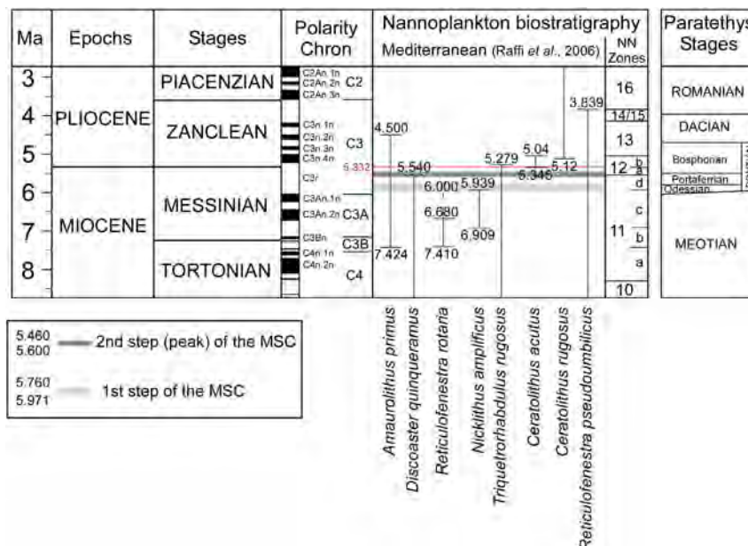
Figure 4. Standard global nannoplankton bio-chronostratigraphy (Raffi et al., 2006) with respect to the Global Polarity Time Scale (Lourens et al., 2005) from 8.5 to 3 Ma. NN Zones are from Martini (1971) amended by Perch-Nielsen (1985) and Berggren et al. (1995). See also Melinte-Dobrinescu et al. (2009) for more details concerning this nannoplankton chart. Correlations with Paratethys Stages are from Vasiliev et al. (2004) and Krijgsman et al. (2010).
