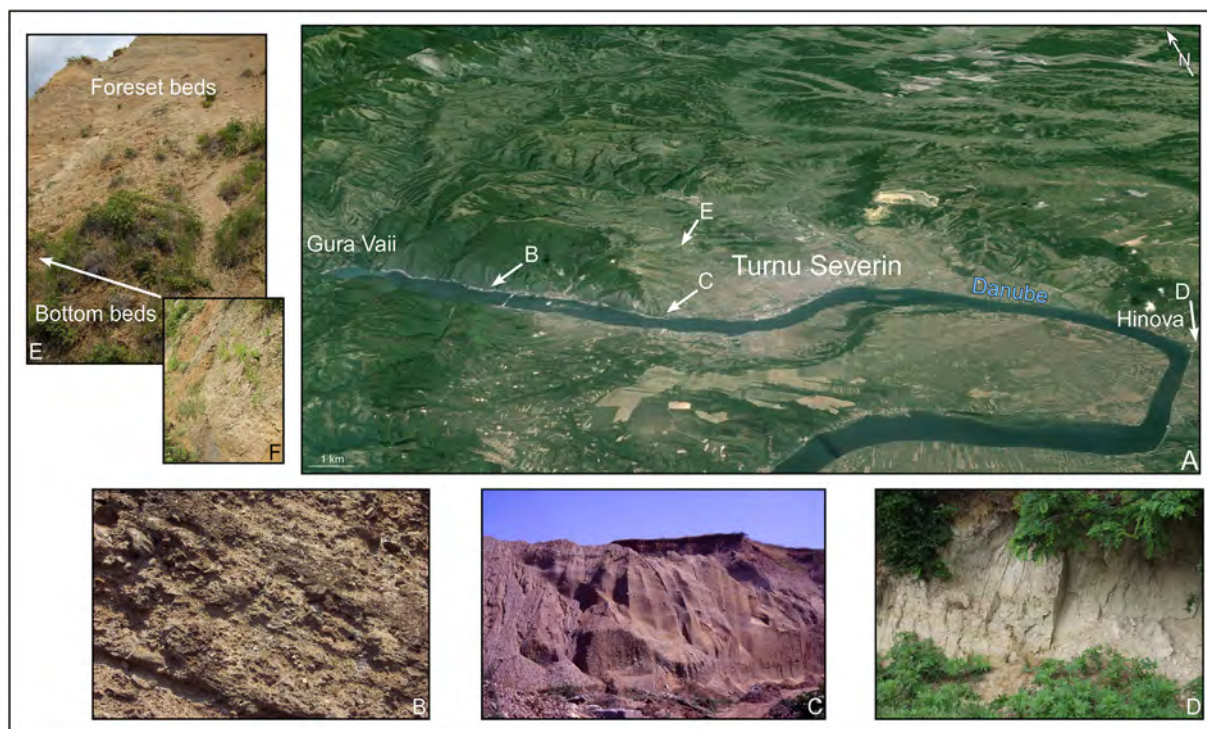
Figure 12. Major features of the Turnu Severin Gilbert-type fan delta. A, GoogleEarth three-dimensional view showing the location of the illustrated sections (relief is exaggerated three times). B, Detail of the conglomeratic foreset beds. C, Gravely and sandy foreset beds. D, Clayey bottomset beds. E, Interlocked bottomset and foreset beds at Pd. Trestenic. F, Detail of the clayey bottomset beds.
