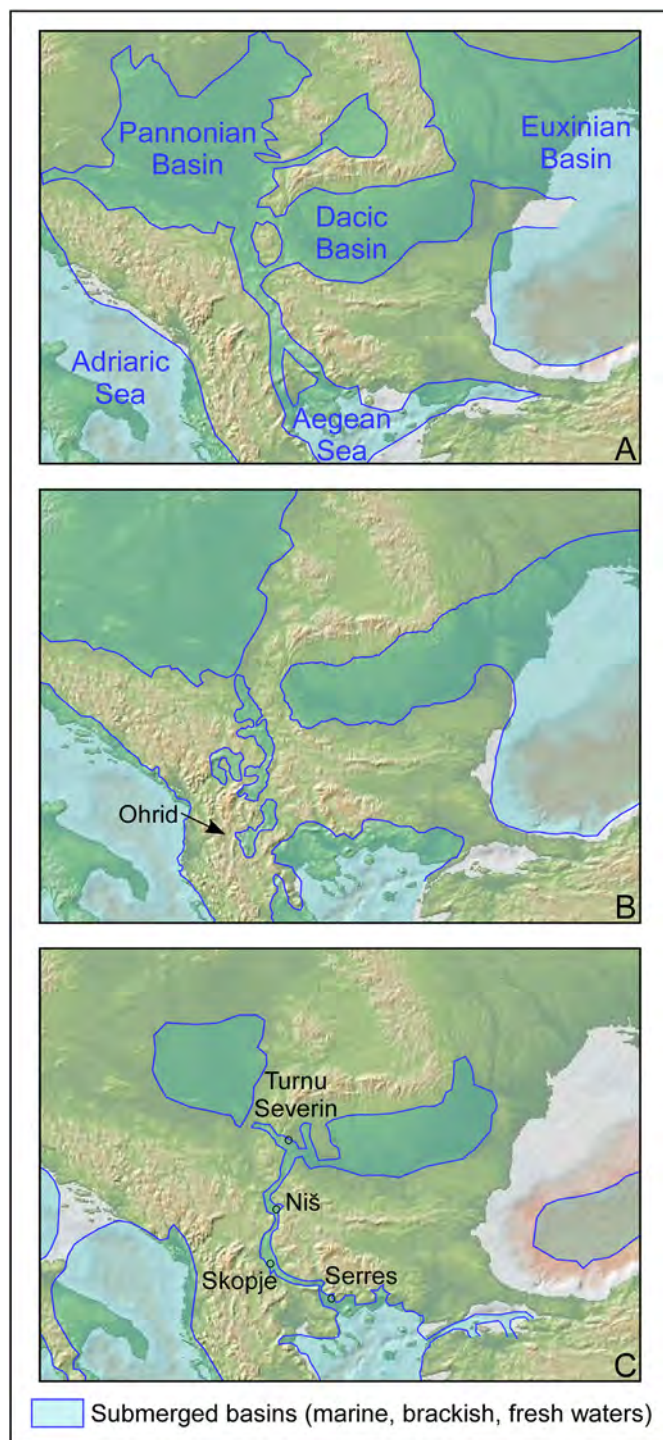
Figure 2. Previously mapped gateways within the Balkans. A, According to Hsü (1978). B, According to Hsü et al. (1977, 1978b). C, According to Bache et al. (2012). Relief is from GeoMapApp® System http://www.geomapapp.org/ (Ryan et al., 2009).
