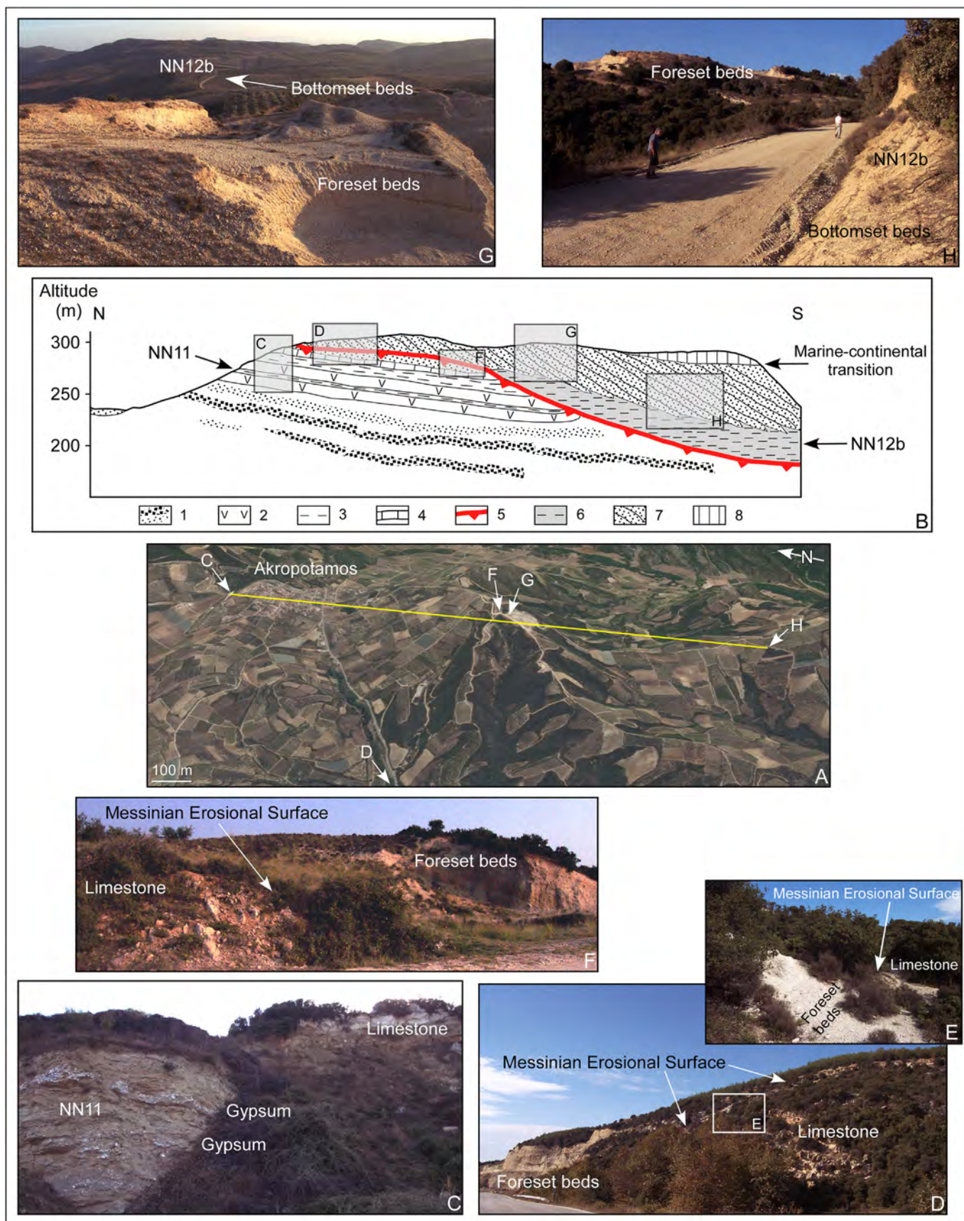
Figure 5. Record of the MSC at Akropotamos (Northern Aegean). A, GoogleEarth three-dimensional view showing the location of the studied section (yellow line) and localities near Akropotamos (relief is exaggerated three times). B, Interpretative sketch of the Akropotamos section. 1, Miocene continental deposits (sands, conglomerates); Messinian: 2,
