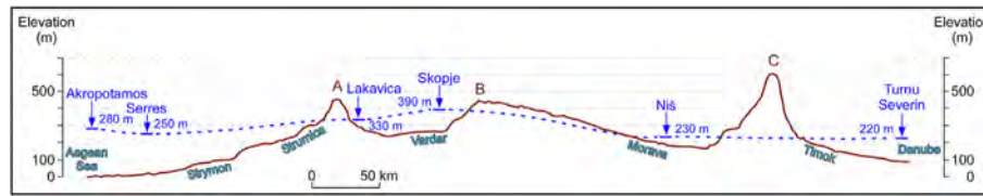
Figure 14. Present-day altitudinal profile of the proposed Balkans corridor with highest places corresponding to the drainage divides (A, between the Strymon and Vardar systems; B, between the Vardar and Morava systems; C, between the Morava and Timok systems) on which is reported the present-day altitude envelope (in blue) of the marine-continental transition (i.e., the Zanclean seashore) in the six evidenced Zanclean deltaic systems. (For interpretation of the references to colour in this figure legend, the reader is referred to the web version of this article.)
