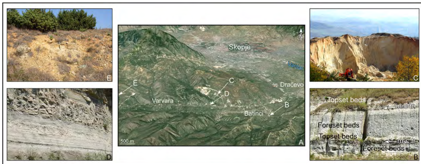
Figure 9. The Dračevo Zanclean Gilbert-type fan delta. A, Skopje area: GoogleEarth three-dimensional view showing the location of the Dračevo Zanclean Gilbert-type fan delta with exposed sections near Batinci and Varvara (relief is exaggerated three times). B, Double marine-continental transition. C, Sandy to conglomeratic foreset beds. D, Clayey bottomset beds. E, Conglomeratic topset beds with travertine blocks.
