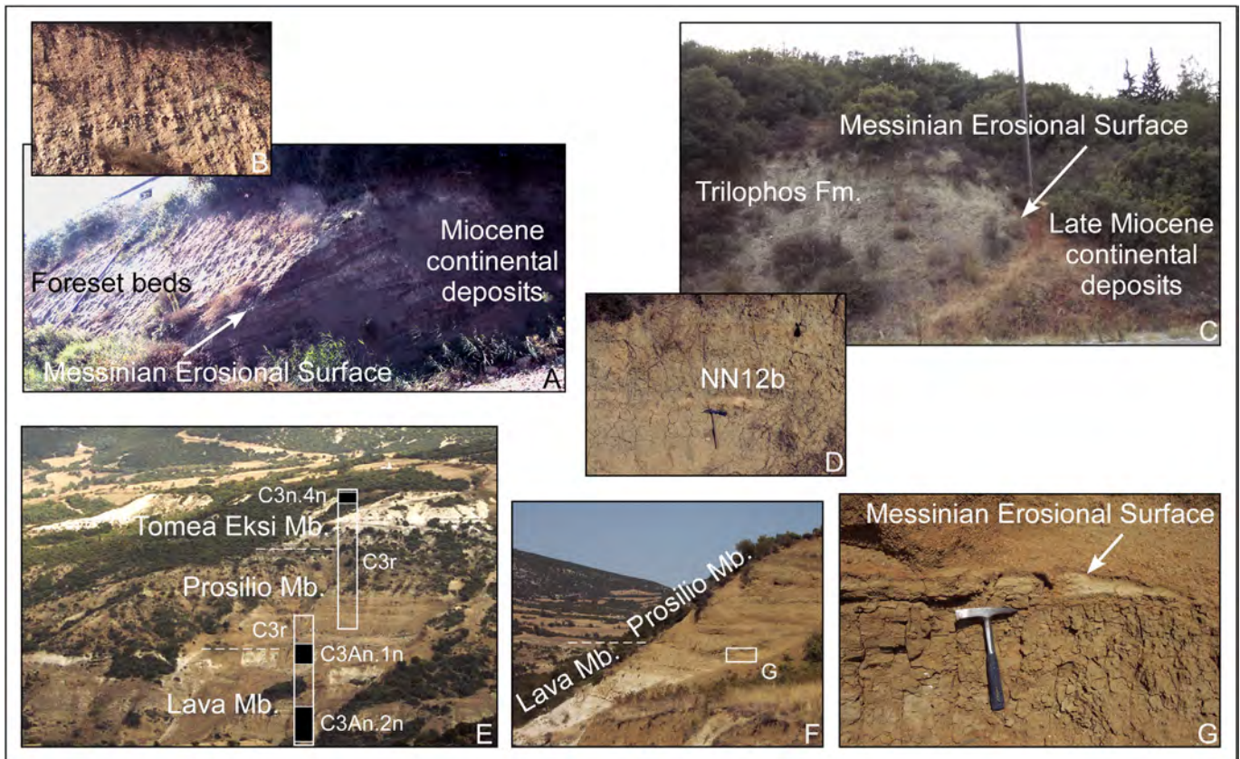
Figure 6. Examples of the Messinian Erosional Surface. A, Near the statue of the Amphipolis Lion. B, Detail of the foreset beds at the same place. C, Near Trilophos. D, Marine clays topping the Trilophos Formation at the same place. E, View of the middle part of the Prosilio section. F, Detail of the same section. G, Detail of photograph F.
