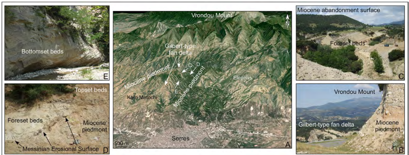
Figure 8. The Serres area. A, GoogleEarth three-dimensional view showing the location of the Serres Zanclean Gilbert-type fan delta nested within the Miocene piedmont of the Vrontou Mount (relief is exaggerated three times). B, View of the foreset beds of the Serres Zanclean Gilbert-type fan delta nested within the Miocene piedmont. C, Zoom on the foreset beds of the Serres Zanclean Gilbert-type fan delta nested within the Miocene piedmont. D, The Messinian Erosional Surface. E, Bottomset beds with lignite beds of the Serres Zanclean Gilbert-type fan delta.
