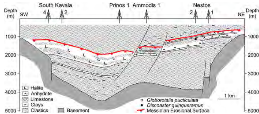
Figure 7. Re-interpreted synthetic section through the Prinos hydrocarbon field (from Proedrou and Sidiropoulos, 1993).
