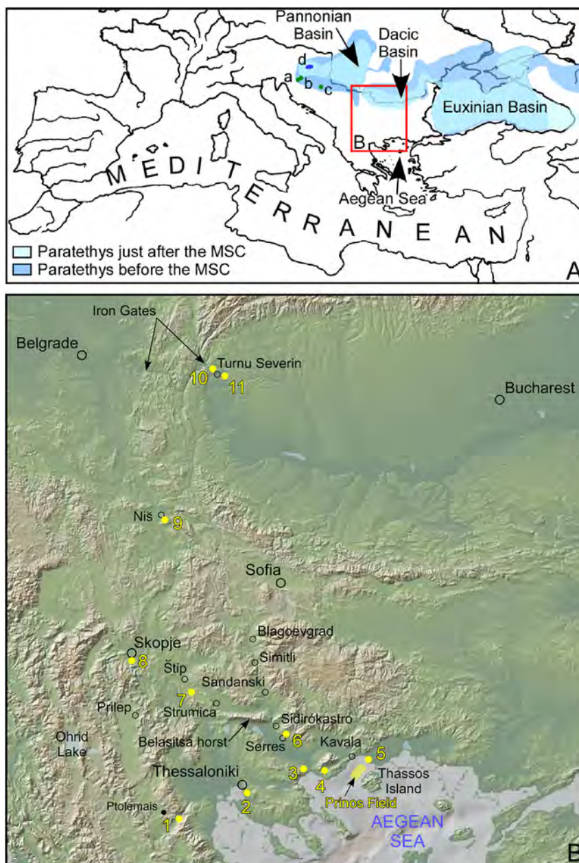
Figure 1. Location maps. A, Location of the study area. Palaeogeography of the Central and Eastern Paratethys before and just after the Messinian Salinity Crisis is from Krijgsman et al. (2010), modified. Proposed gateway(s), subject of this paper, are not shown. Pannonian – Early Pontian quoted localities: a, Krasčić; b, Malunje; c, Krasjčići. Pannonian – Late Pontian quoted locality: d, Mura-Zala Basin. B, Studied localities. 1, Proslilio; 2, Trilophos; 3, Amphipolis Lion; 4, Akropotamos; 5, Nestos 1 and 2 wells; 6, Serres; 7, Lakavica; 8, Dračevo; 9, Gabrovačka; 10, Gura Vajii – Turnu Severin; 11, Hinova. Relief is from GeoMapApp® System http://www.geomapp.org/ (Ryan et al., 2009).
