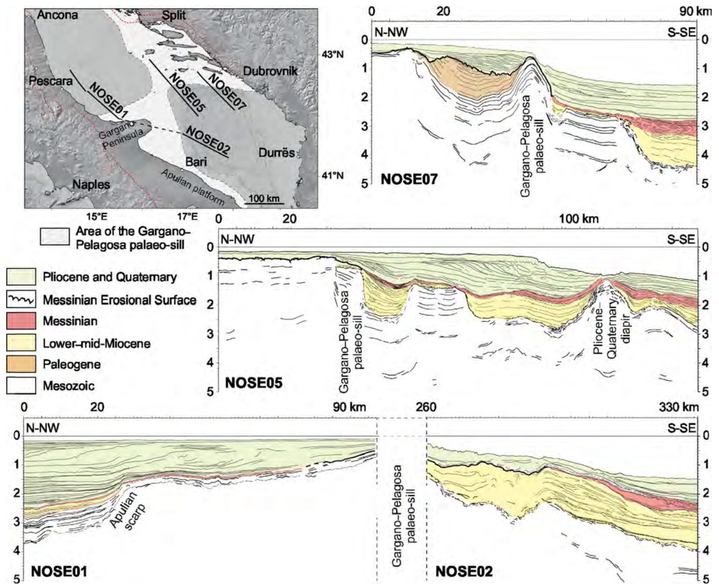
Fig. 16. Line drawings of interpreted seismic profiles in the Adriatic Sea showing the Messinian Gargano–Pelagosa palaeo-sill.
