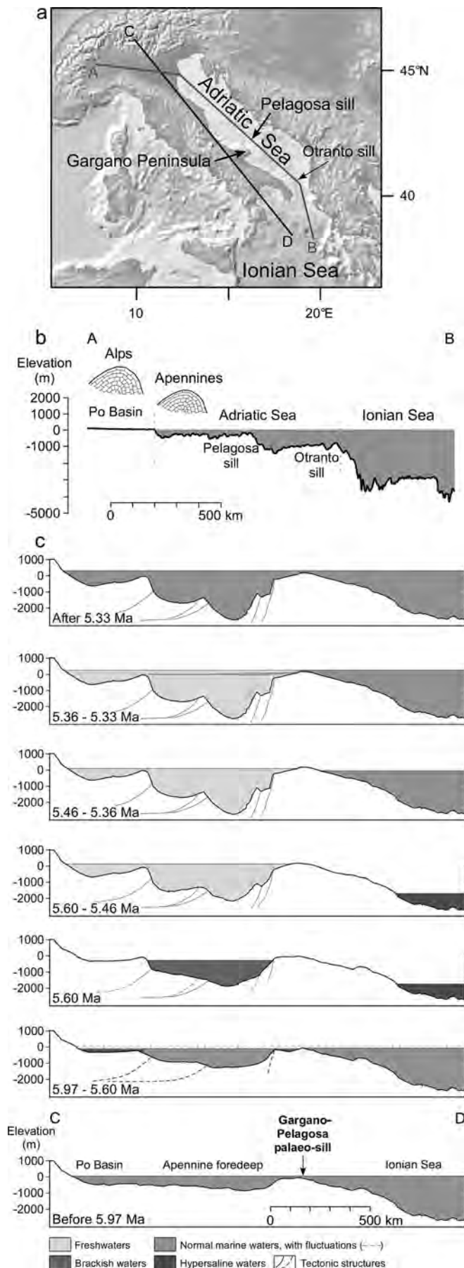
Fig. 15. Mediterranean–Adriatic (vs. Apennine foredeep) connections since 6 Ma: a : location of the cross-sections; b : present-day cross-section; c : successive reconstructed cross-sections from 5.97 to 5.33 Ma, highlighting the role of the Gargano–Pelagosa palaeo-sill and Messinian Apennine deformation phase.
