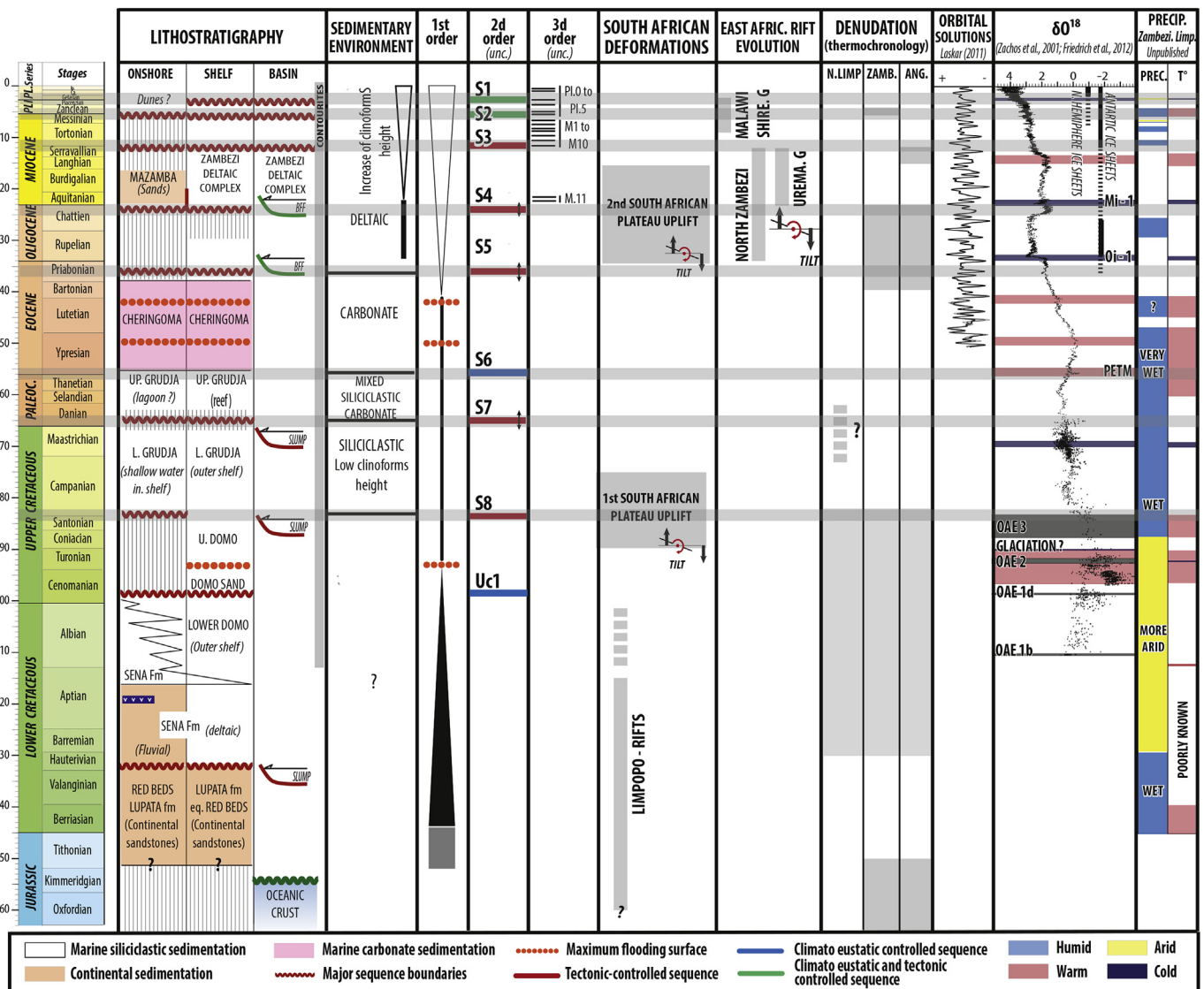
Fig. 12. Summary chart of the stratigraphic data and their possible causes, deformations and climates.
