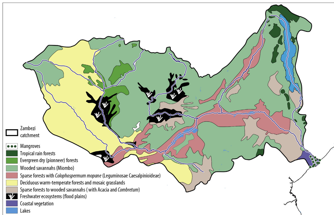
Fig. 3. Present day vegetation distribution within the Zambezi catchment (Timberlake, 2000).
