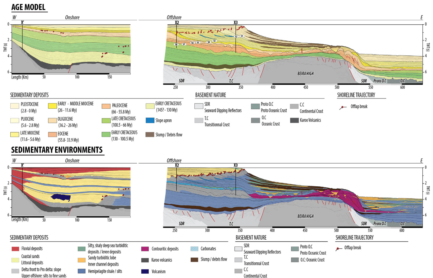
Fig. 6. Zambezi Delta regional seismic line from the upstream coastal plain bordered by the Cheringoma Plateau to the Beira High (see location on Fig. 1B): age model and sedimentary environments.
