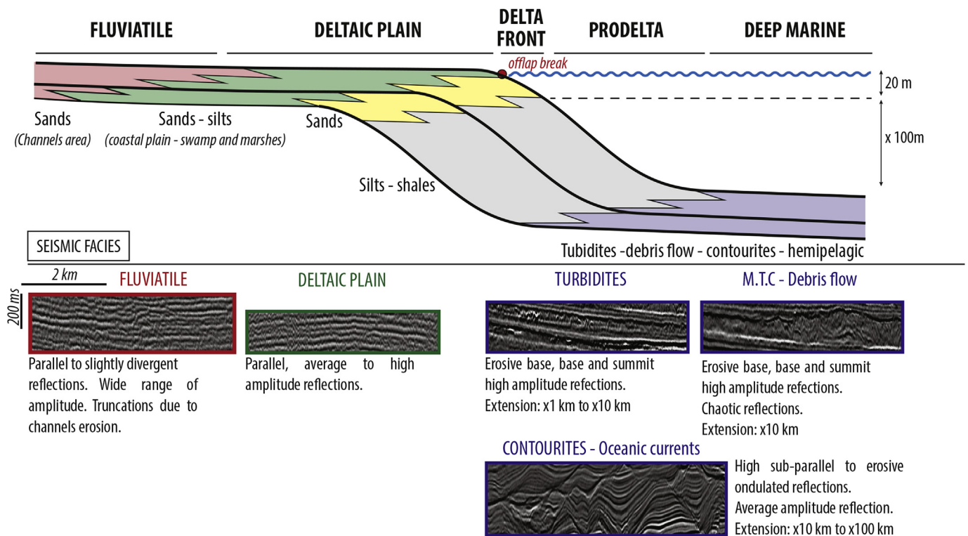
Fig. 5. Margin delta depositional profile: environments and lithology, clinoforms height and main seismic facies.
