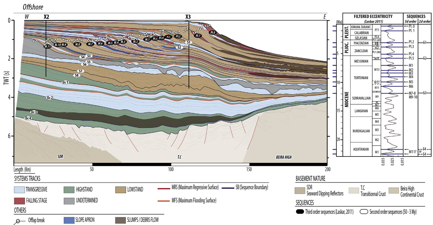
Fig. 10. Age model for Zambezi Delta Neogene sediments: (1) repetitive unconformity-bounded third-order depositional sequences influenced by climate-induced sea level changes, defined on both offlap break migration and stratigraphic truncations (labelled from Pl.0 to Pl.5 and M.1 to M.11) and (2) calibration of the third-order sequence boundaries on Laskar's orbital solution (eccentricity; Laskar et al., 2011) based on the assumption that a sea level fall must correspond to a major cooling and therefore to a decrease in eccentricity.
