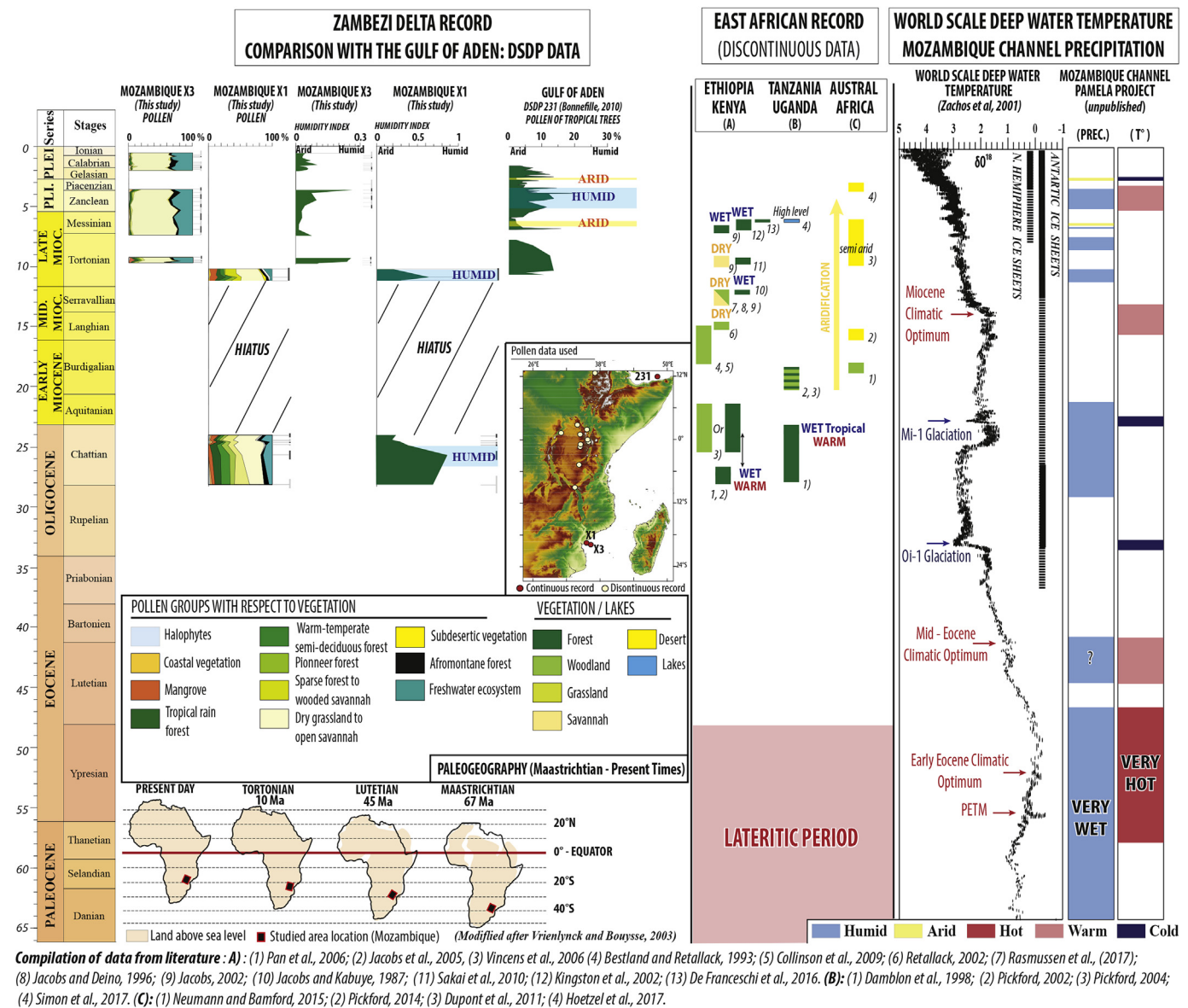
Fig. 11. Reconstructed precipitation estimates of the Zambezi catchment from the Oligocene up to Present in the frame of the East Africa: (1) from wells X1 and X3 (see Fig. 1B for location) based on pollen records (this study see text for discussion) and comparison with the reference DSDP Site 231 (Gulf of Aden; Bonnefille, 2010 ); (2) compilation of the published precipitation evaluation from scattered outcrops in East Africa mainly based on palaeobotanical data (woods, leaves, pollen grains), (3) regional (Mozambique Channel) and world-scale climatic data. The Mozambique Channel data (unpublished at the moment) were acquired in the frame of the PAMELA Project through a collaboration between geoscientists of Rennes University and palynologists of TOTAL Company (N. Buratti and D. Michoux).
