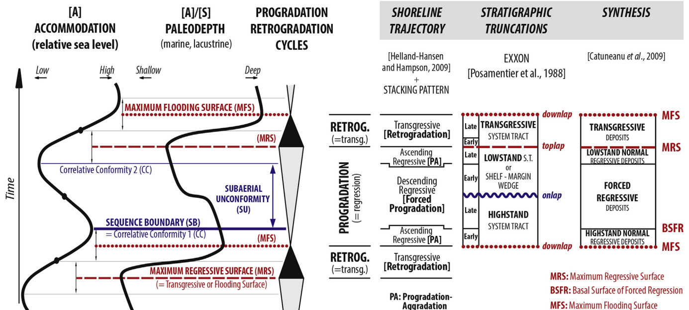
Fig. 2. Summary chart of approaches used to interpret seismic stratigraphy.
