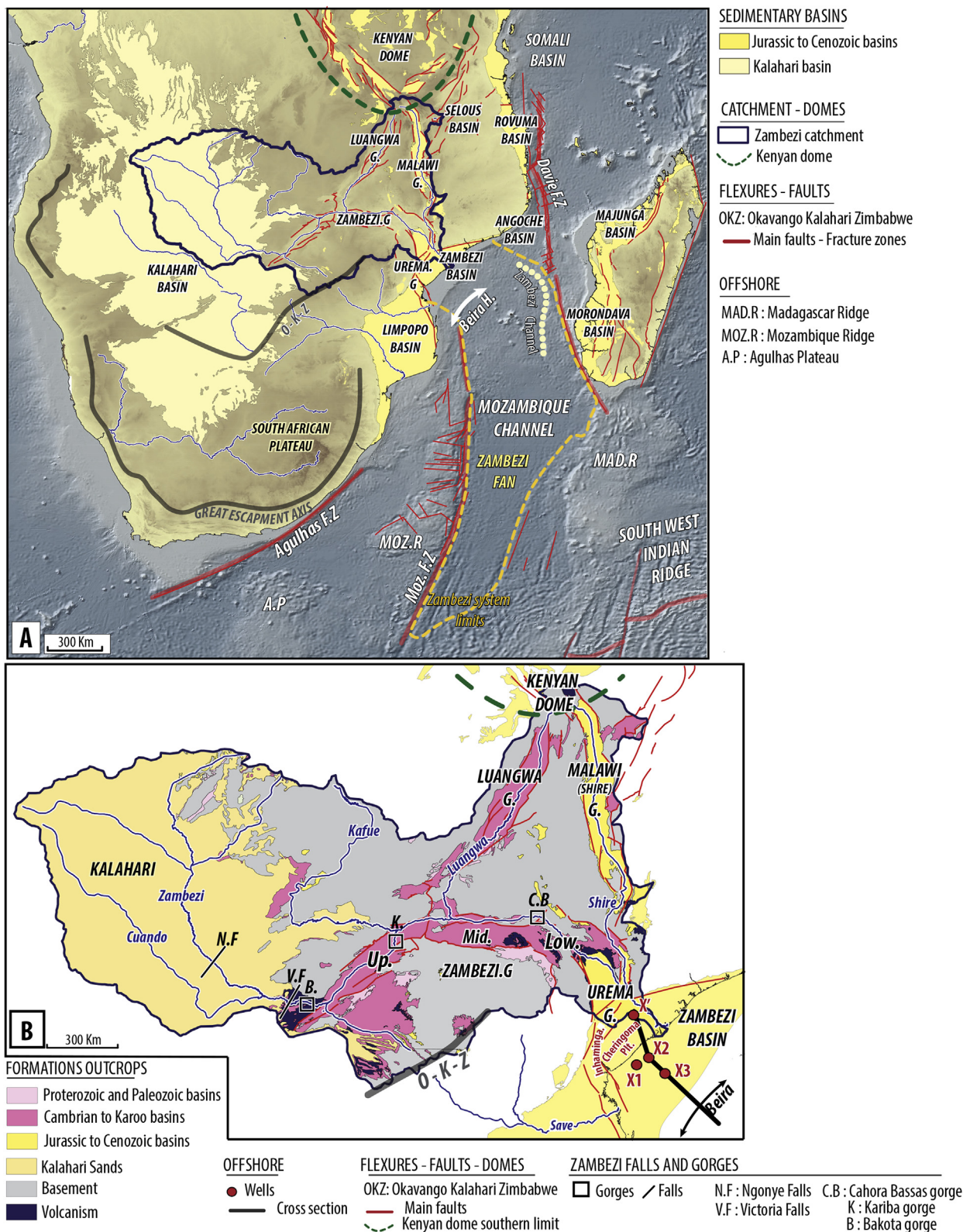
Fig. 1. The Zambezi sedimentary system. A: Location in Austral Africa (catchment) and in the Mozambique Channel (deep-sea fan). B: Main geological features of the catchment (Cenozoic Kalahari Basin, Late Carboniferous to Triassic Karoo rifts, Neogene rifts and main faults).
