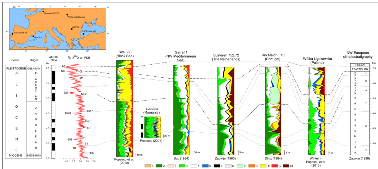
Fig. 1 - Example of climatostratigraphic correlations at the European scale between six long pollen records from the earliest Pliocene to earliest Pleistocene and chronologic calibration of the Northwestern European climatic succession (modified from Popescu et al., 2010). Pollen groups (thermic classification: Nix, 1982): 1, Megathermic elements ( Canthium , Sapindaceae, Bombax , etc.); 2, Mega-mesothermic elements ( Taxodium -type, Sequoia -type, Arecaceae, Engelhardia , Distylium , Microtropis fallax , etc.); 3, Cathaya (= Pinus haploxylon-type at Wólka Ligezawska); 4, Mesothermic elements ( Quercus , Carya , Pterocarya , Liquidambar , Carpinus , Ulmus , Zelkova , etc.); 5, Pinus ; 6, Meso-microthermic trees ( Cedrus , Tsuga , Keteleeria ); 7, Microthermic trees ( Abies , Picea ); 8, Elements of no significance (Ranunculaceae, Rosaceae, etc.); 9, Cupressaceae ( Cupressus - Juniperus -type); 10, Mediterranean xerophytes ( Olea , Pistacia , Ceratonia , Quercus ilex -type, Rhamnus , Cistus , etc.); 11, Herbs (Amaranthaceae, Asteraceae, Poaceae, Apiaceae, Rumex , Boraginaceae, Convolvulus , Cyperaceae, Caryophyllaceae, etc.); 12, Steppe elements ( Artemisia , Ephedra , Hippophae ); 13, Ericaceae.
