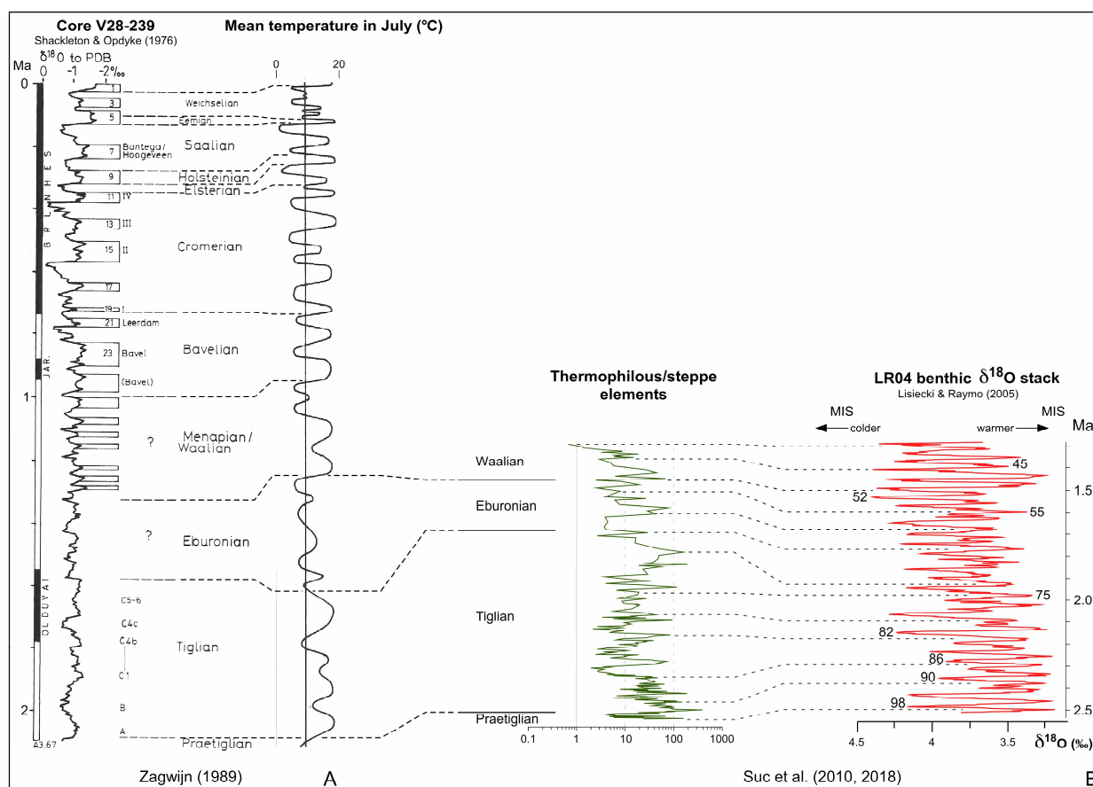
Fig. 3 - Climatic curves resulting from pollen records compared to oxygen isotope curves. A) The Netherlands climatic curve matched to an oxygen isotope curve (modified from Zagwijn, 1989); B) Focus on the latest Praetiglian to early Waalian pollen ratio 'thermophilous/steppe elements' from the Mediterranean region (Croton, Calabrian Stage) compared with the LR04 benthic \delta^{18}\text{O} stack (modified from Suc et al., 2010, 2018).
